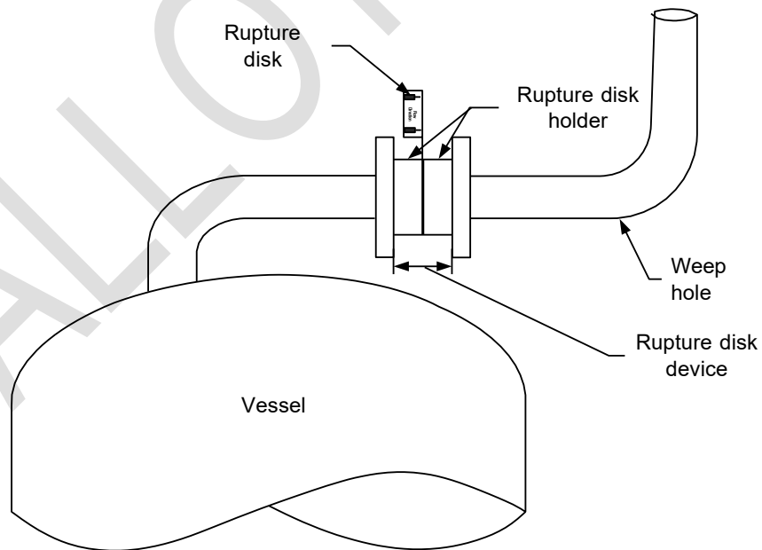
Figure 4a—Typical Rupture Disk Device Installation: Atmospheric (Open) Discharge
