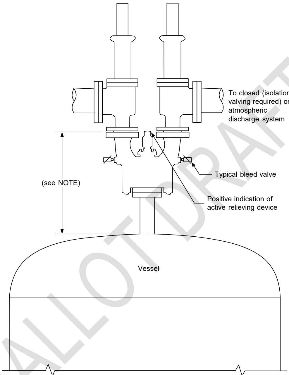
Figure 12—Alternate PRD Installation for 100 % Spare Relieving Capacity
