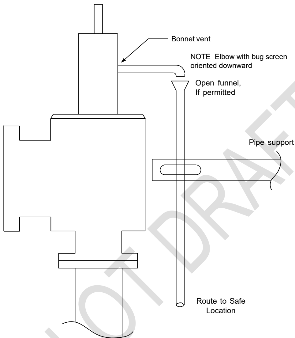
Figure 21— Bonnet Vent for Bellows Valves Handling Non-Hazardous Liquids Where a Leak Needs to the Vent is Be Routed Away from the PRV
