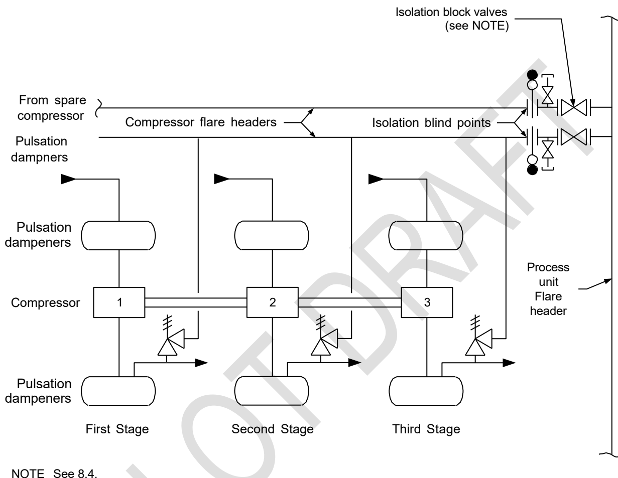
Figure 17—Typical Isolation Block Valves for Spare Compressor
