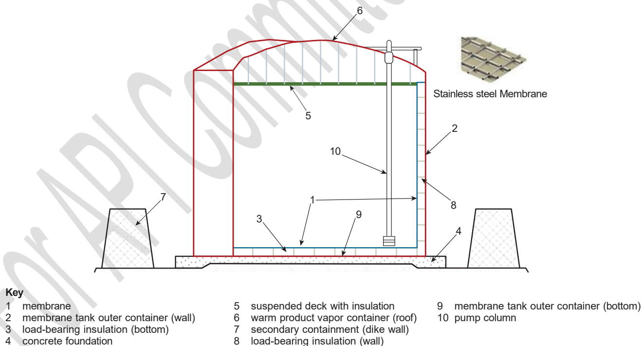
Figure 13—Membrane Containment Tank System Type M-1: Membrane with Steel Membrane Tank Outer Container
