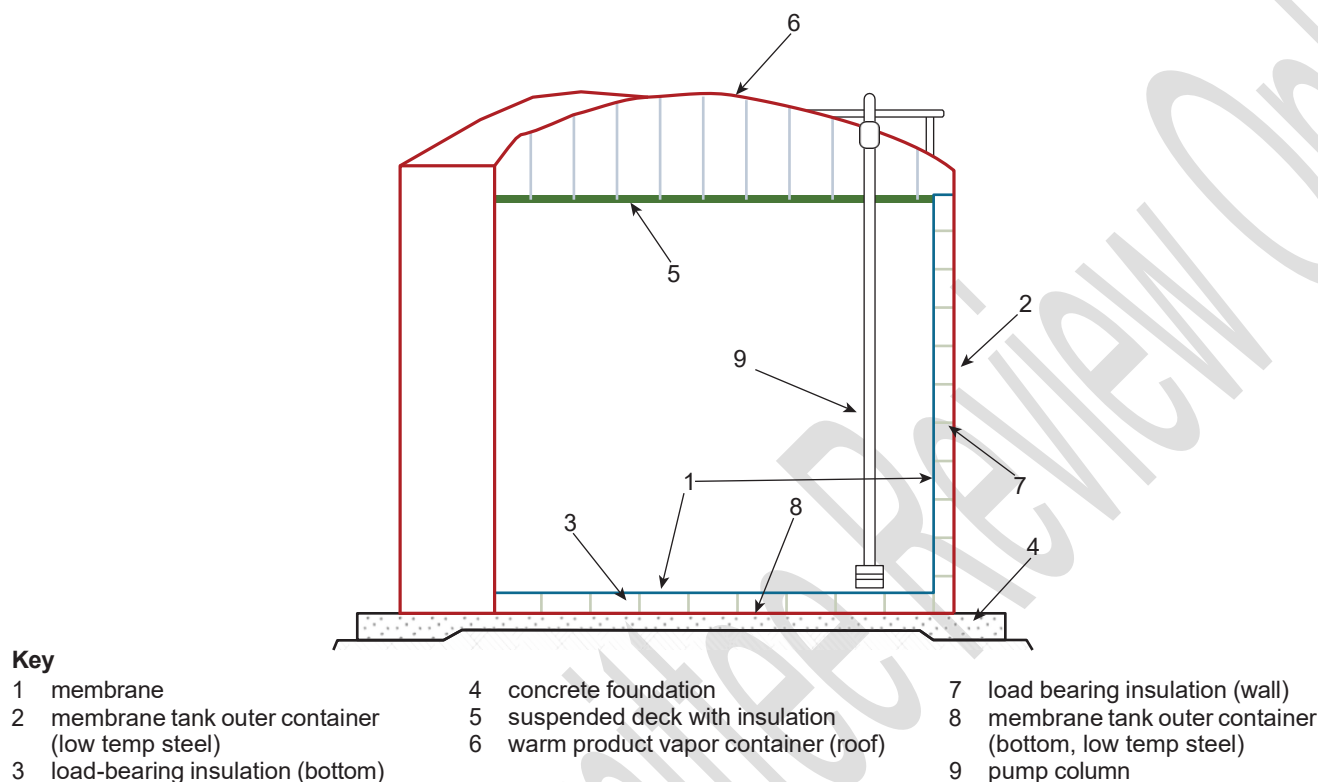
Figure 14—Membrane Containment Tank System Type M-CC: Membrane with Steel Membrane Tank Outer Container
