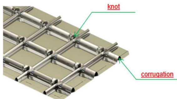
Figure 1—Example of Corrugations on the Membrane
