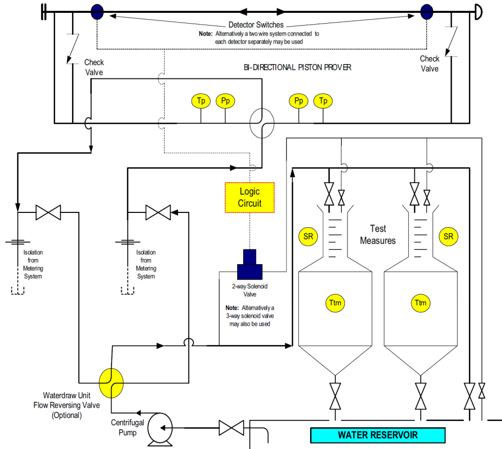
Figure D.2A—Schematic Drawing of a Typical Layout for a Waterdraw Calibration of a Displacement Type Bi-directional Prover with a Free Piston Displacer and Check Valves in the Manifold using Top-filling Test Measures
