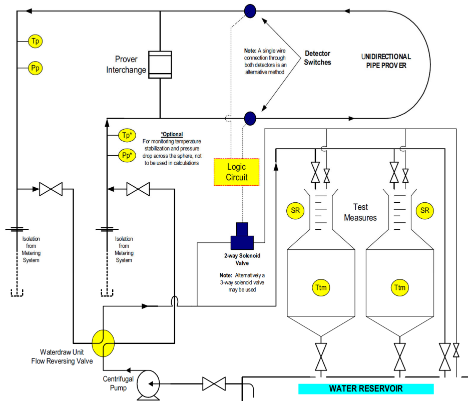
Figure D.1—Schematic Drawing of a Typical Layout for a Waterdraw Calibration of a Displacement Type Unidirectional Prover with a Free Displacer using Top-filling Test Measures
