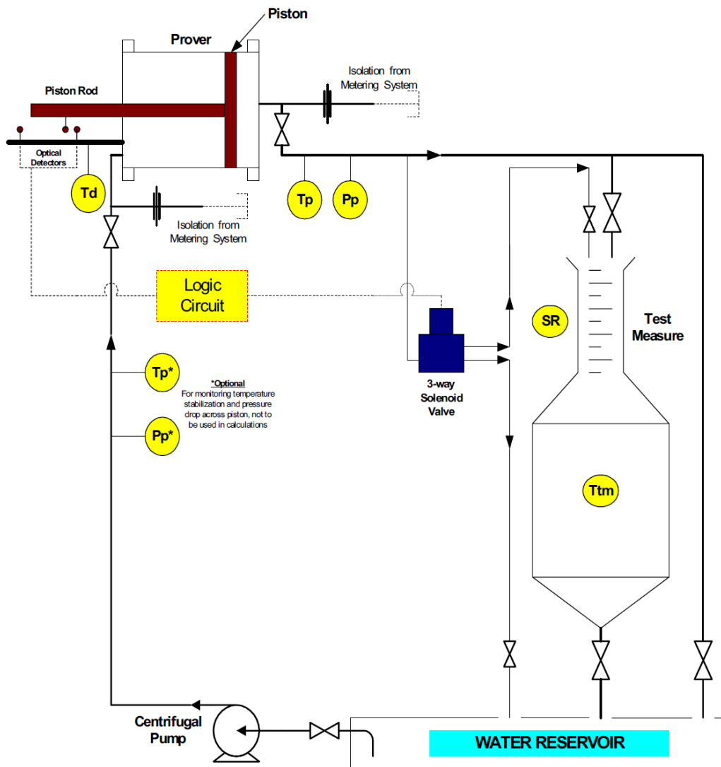
Figure D.3A—Schematic Drawing of a Typical Layout for a Waterdraw Calibration of the Downstream Volume of a Displacement Prover with a Captive Displacer and External Detectors using Top-filling Test Measures
