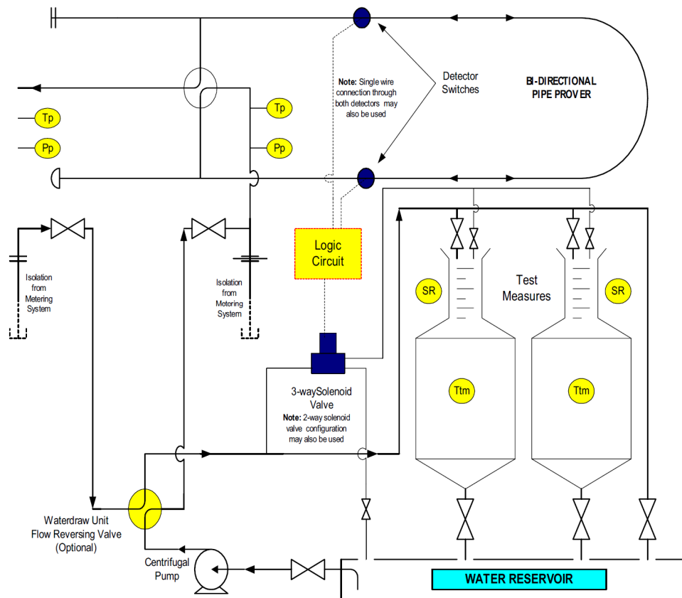
Figure D.2B—Schematic Drawing of a Typical Layout for a Waterdraw Calibration of a Displacement Type Bi-directional Prover with a Free Sphere Displacer using Top-filling Test Measures
