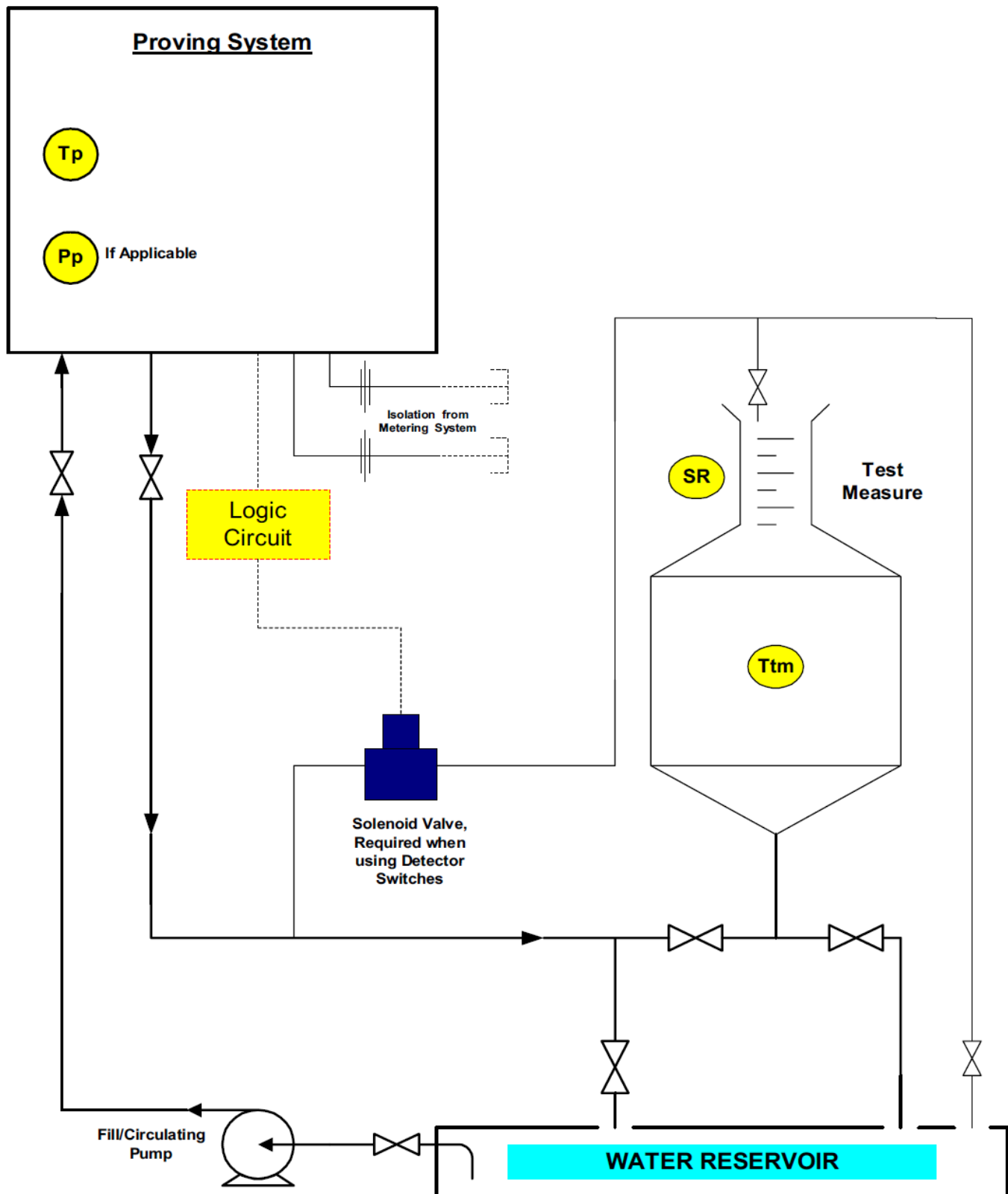
Figure D.5—Alternate Method—Schematic Drawing of a Typical Layout for a Waterdraw Calibration of a Proving System using Bottom-filling Test Measures
