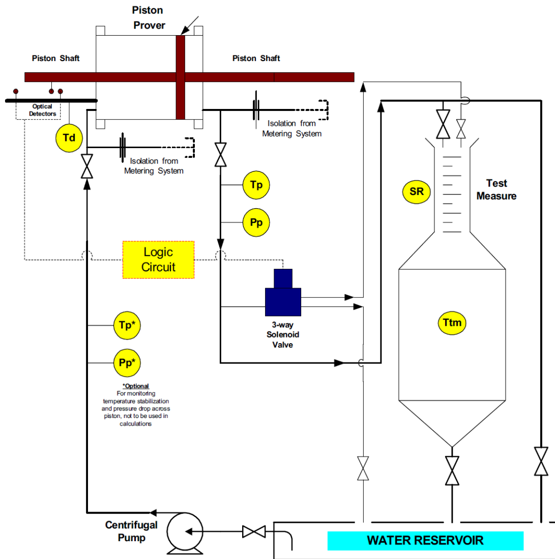
Figure D.3C—Schematic Drawing of a Typical Layout for a Waterdraw Calibration of a Displacement Prover with Equal Size Diameter Shafts on Both Sides of a Captive Displacer and External Detectors using Top-filling Test Measures
