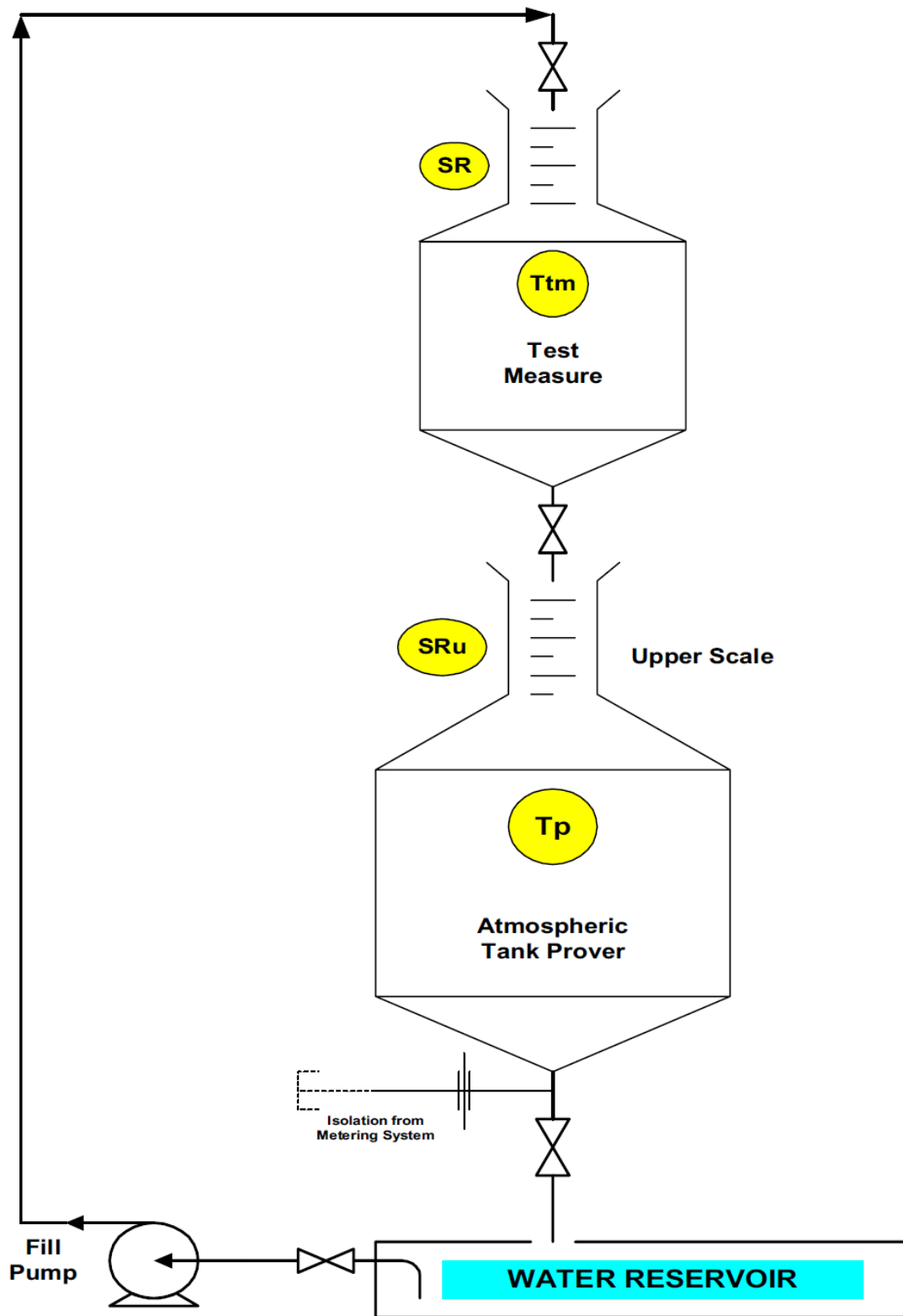
Figure D.4B—Schematic Drawing of a Typical Layout for a Waterdraw Calibration of a Volumetric Tank Prover with a Dry Bottom using the Water-fill Method and using Top-filling Test Measures.
