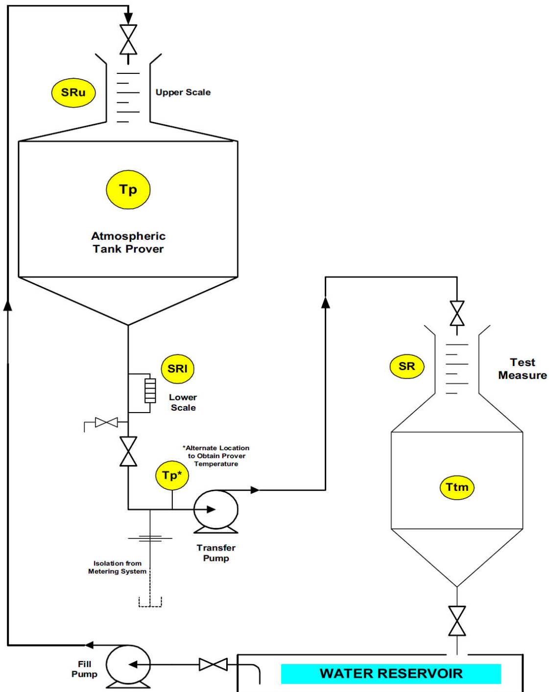
Figure D.4C—Schematic Drawing of a Typical Layout for a Waterdraw Calibration of a Volumetric Tank Prover with a Wet Bottom using Top-filling Test Measures
