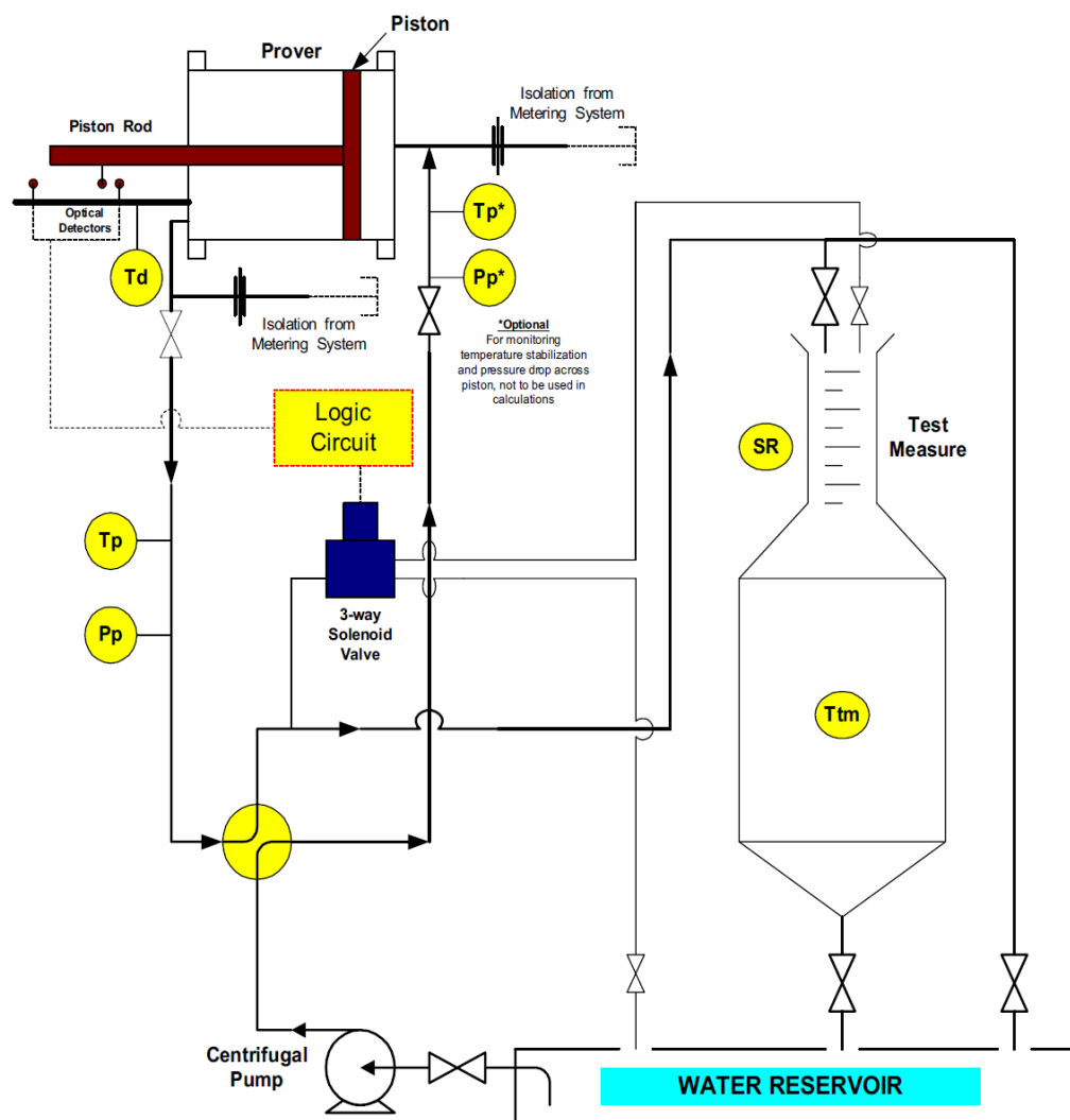
Figure D.3B—Schematic Drawing of a Typical Layout for a Waterdraw Calibration of the Upstream Volume of a Displacement Prover with a Captive Displacer and External Detectors using Top-filling Test Measures
