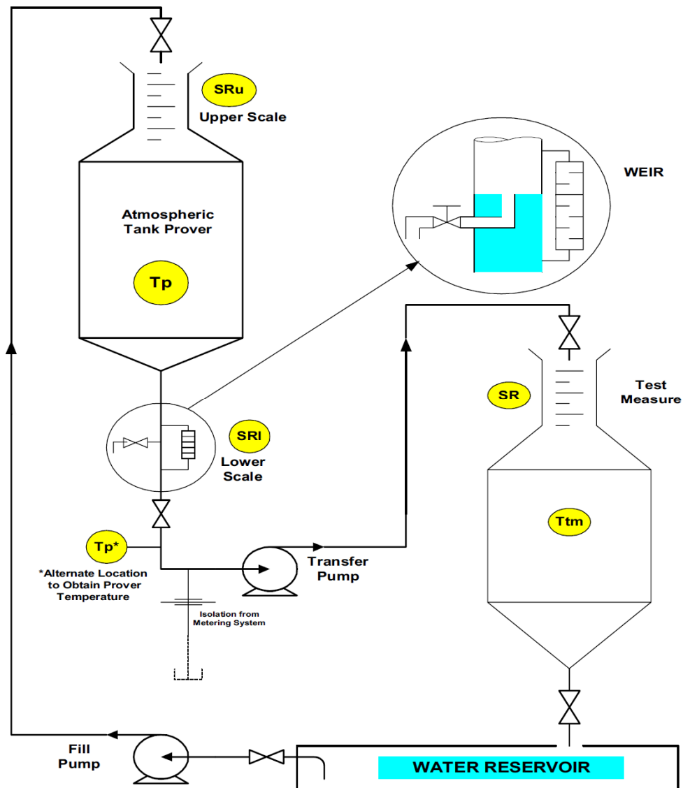
Figure D.4A—Schematic Drawing of a Typical Layout for a Waterdraw Calibration of a Volumetric Tank Prover with a Bottom Weir using Top-filling Test Measures
