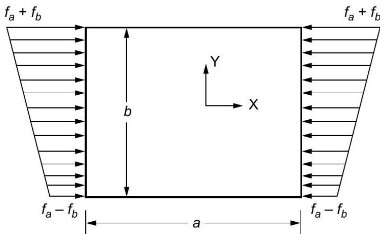
Figure 5.2-1—Long Rectangular Plate
