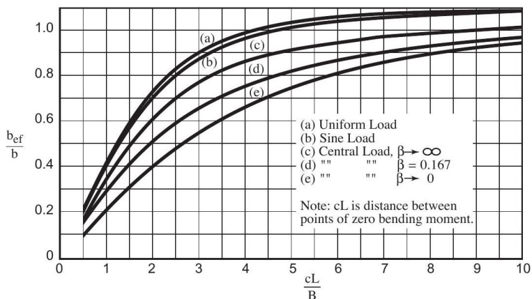
Figure 7.6-4—Effective Breadth Ratio for Case III (Multiple Webs)*
