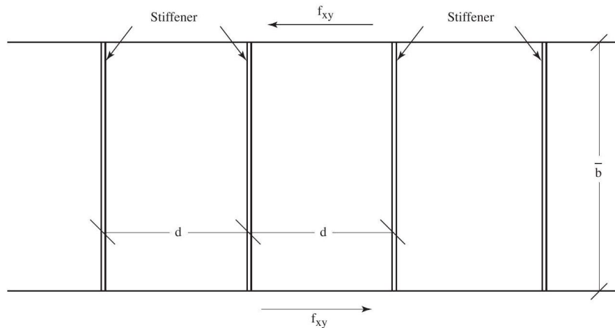
Figure 7.7-1—Geometry of Stiffened Panels Subjected to In-Plane Shear
