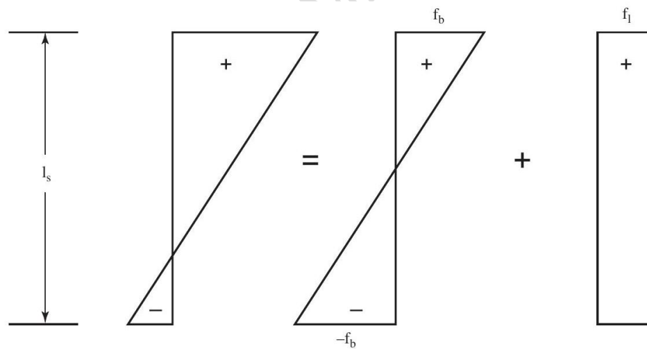
Figure 8.3-5—Longitudinal Stress in Webs with Transverse Stiffeners
