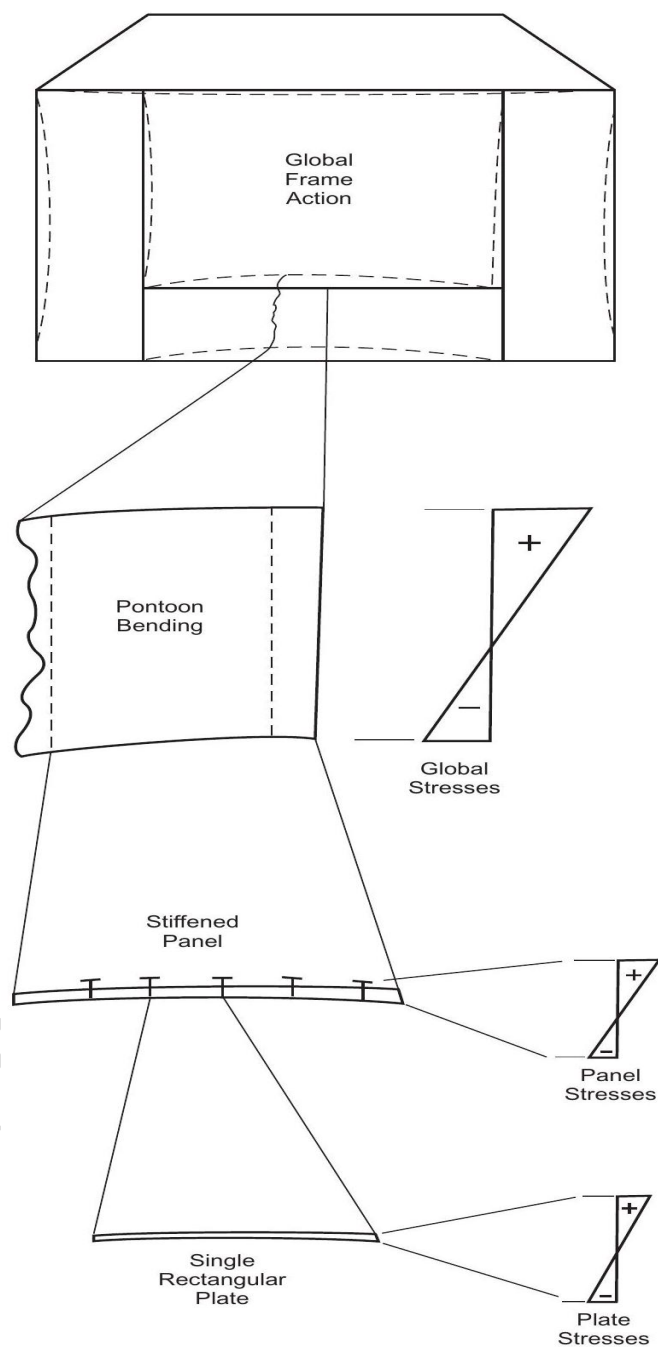
Figure 4.6-1—Global, Panel, and Plate Stresses
