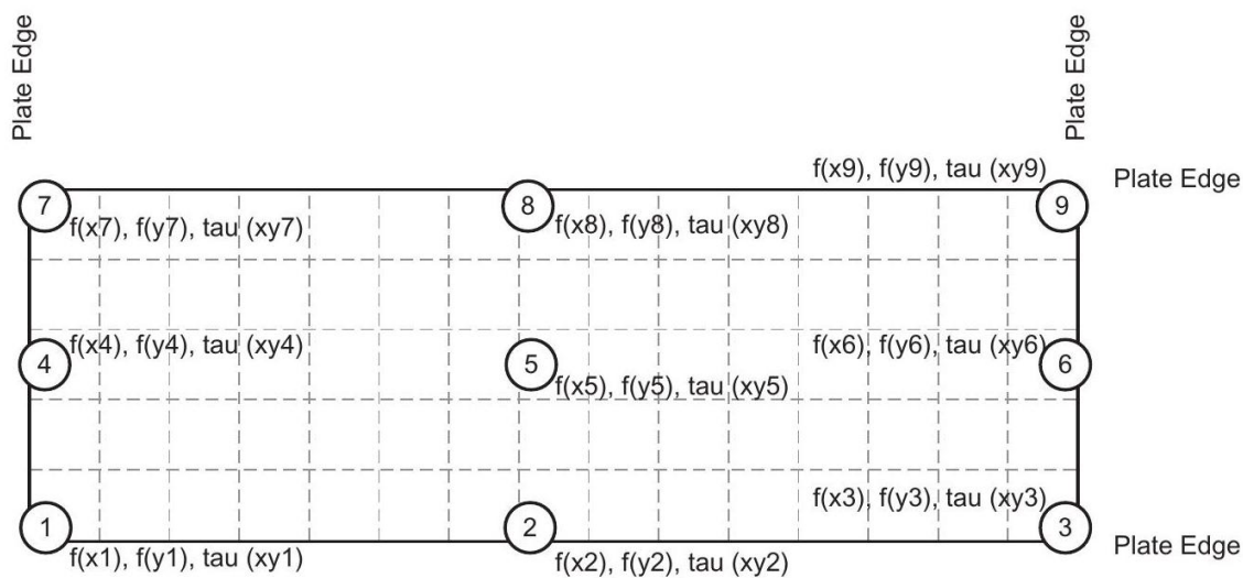
FEA Stress Locations for Rectangular Plate
