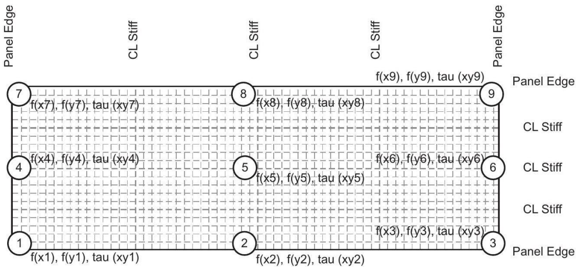
FEA Stress Locations for Rectangular Panel
