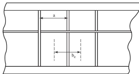
Figure 8.3-2—Web with Large Openings
