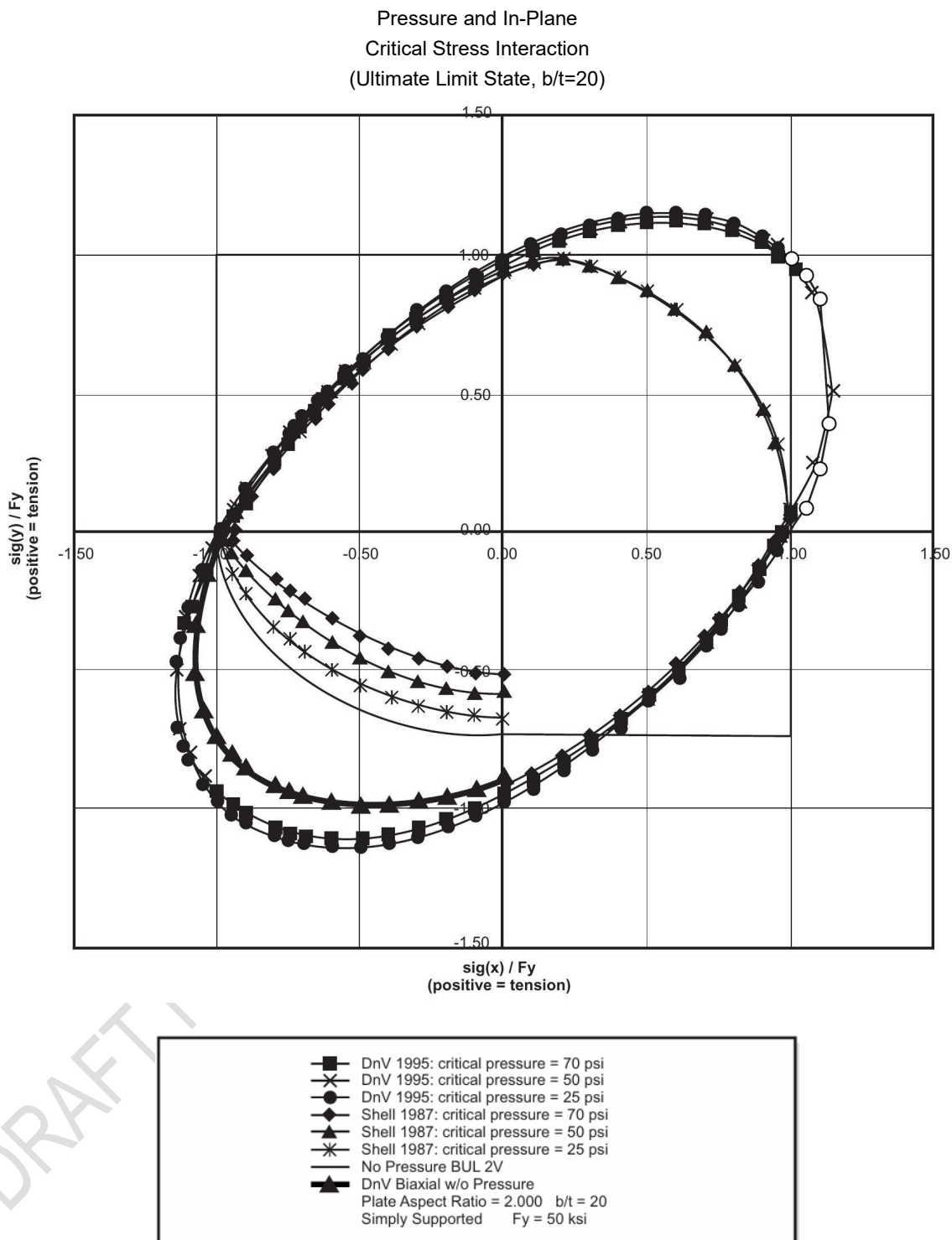
Figure C5-11—Combined In-Plane and Lateral Loads ( b/t = 20 )
