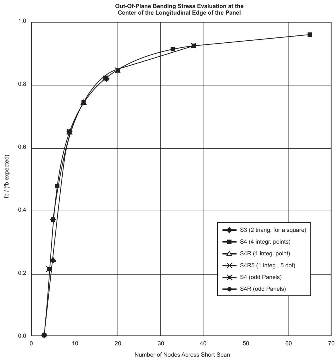
Figure A-2—Panel Weak Axis Bending Stress Evaluation at Center of Longitudinal Edge
