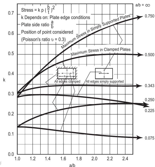
Figure 5.2-4-Stresses in Plates Under Uniform Lateral Pressure 3
