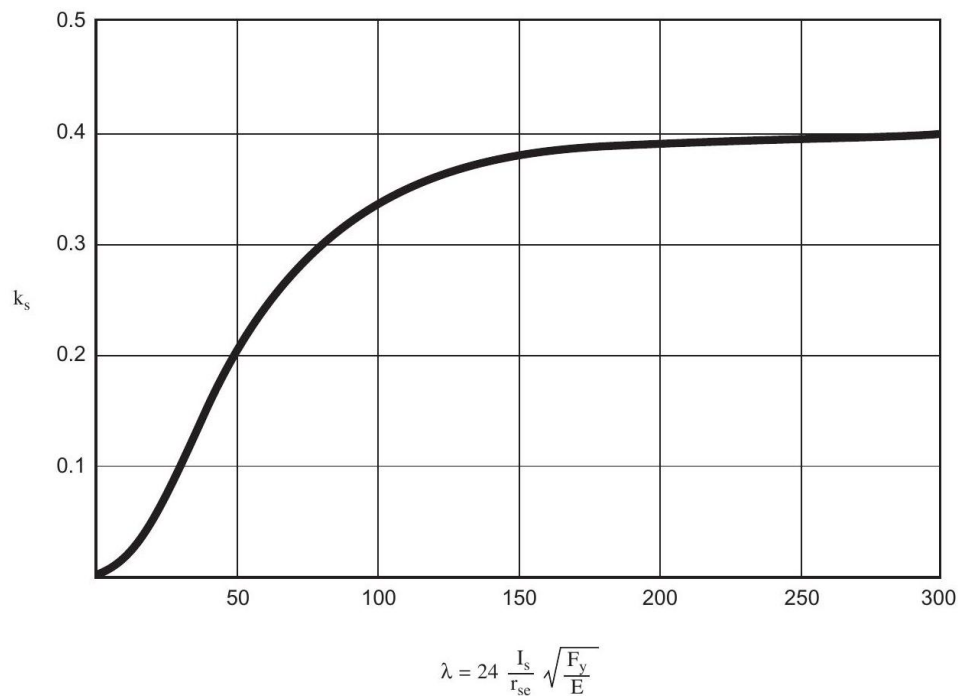
Figure 8.3-4—Coefficient for Computing Axial Force Assumed in Preventing Web Buckling
