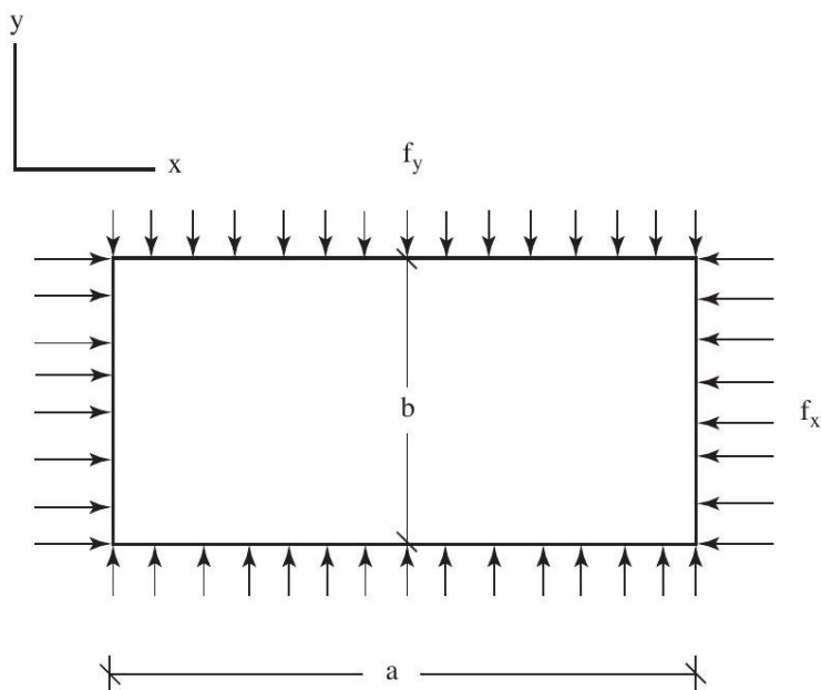
Figure C5-9—Rectangular Plate Under Biaxial Compression
