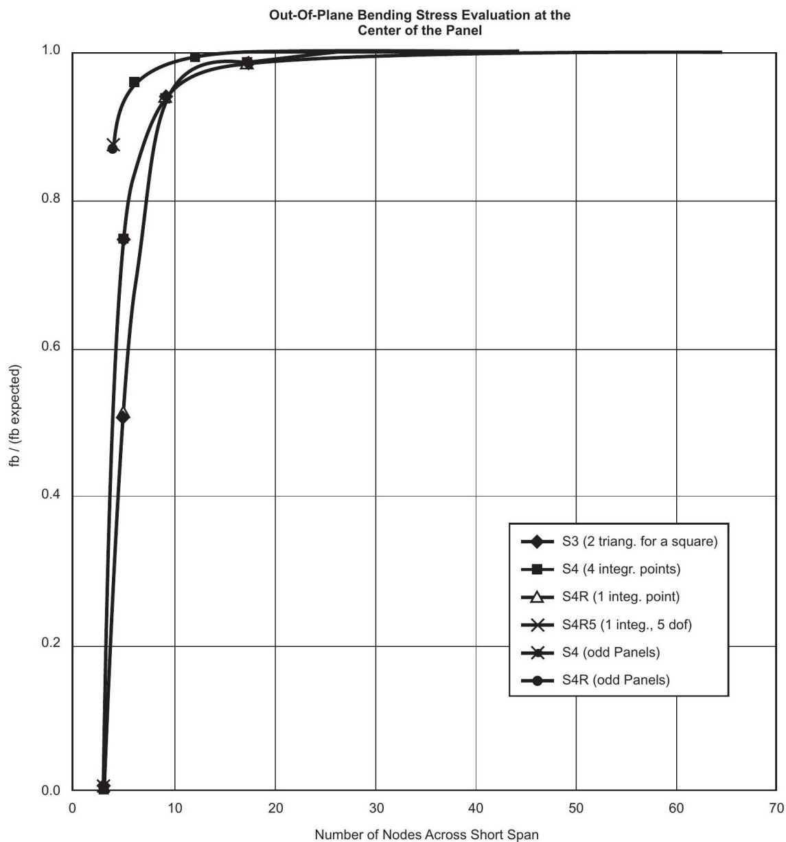
Figure A-1—Panel Weak Axis Bending Stress Evaluation at Center of Panel
