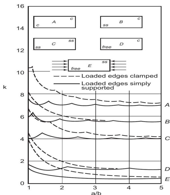
Figure 5.2-3-Buckling Coefficients for Plates in Uniaxial Compression 1
