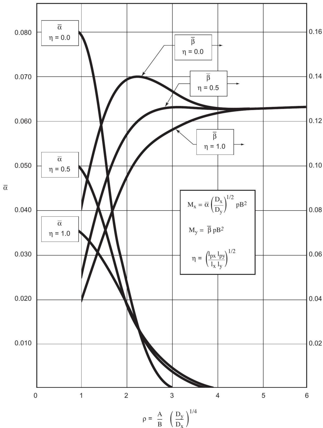
Figure 7.3-2—Coefficients for Computing Stresses for Orthogonally Stiffened Panels
