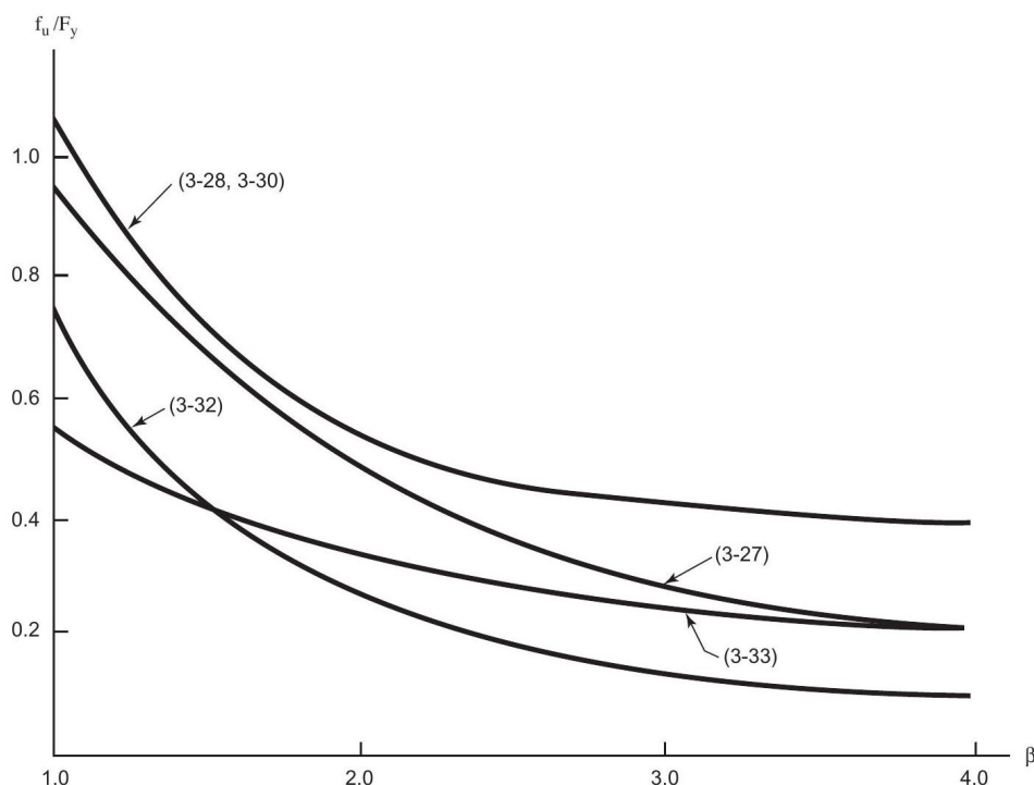
Figure C5-4—Comparison of Formulations for the Ultimate Strength of Wide Plates with a/b = 3
