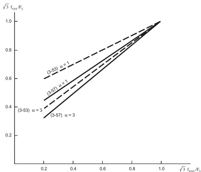
Figure C5-7—Comparison of Formulations for the Ultimate Strength of Rectangular Plates in Shear
