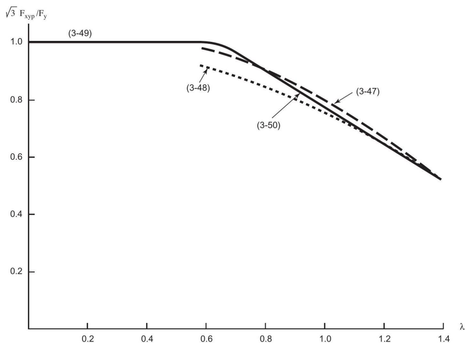
Figure C5-5—Comparison of Formulations for the Inelastic Buckling of Rectangular Plates Under Edge Shear
