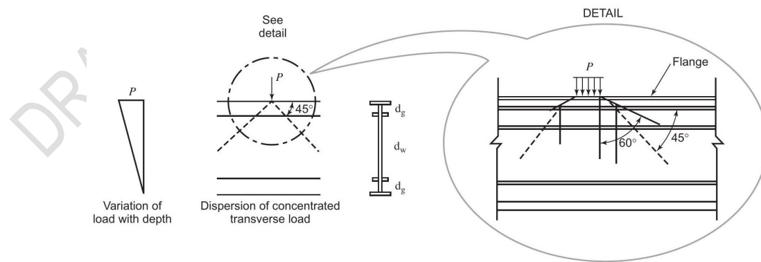
Figure 8.1-3—Stress Distribution Across Section Due to Concentrated Load Applied at the Flange Level
