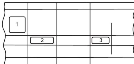
Figure 8.3-1—Web with Small Openings
