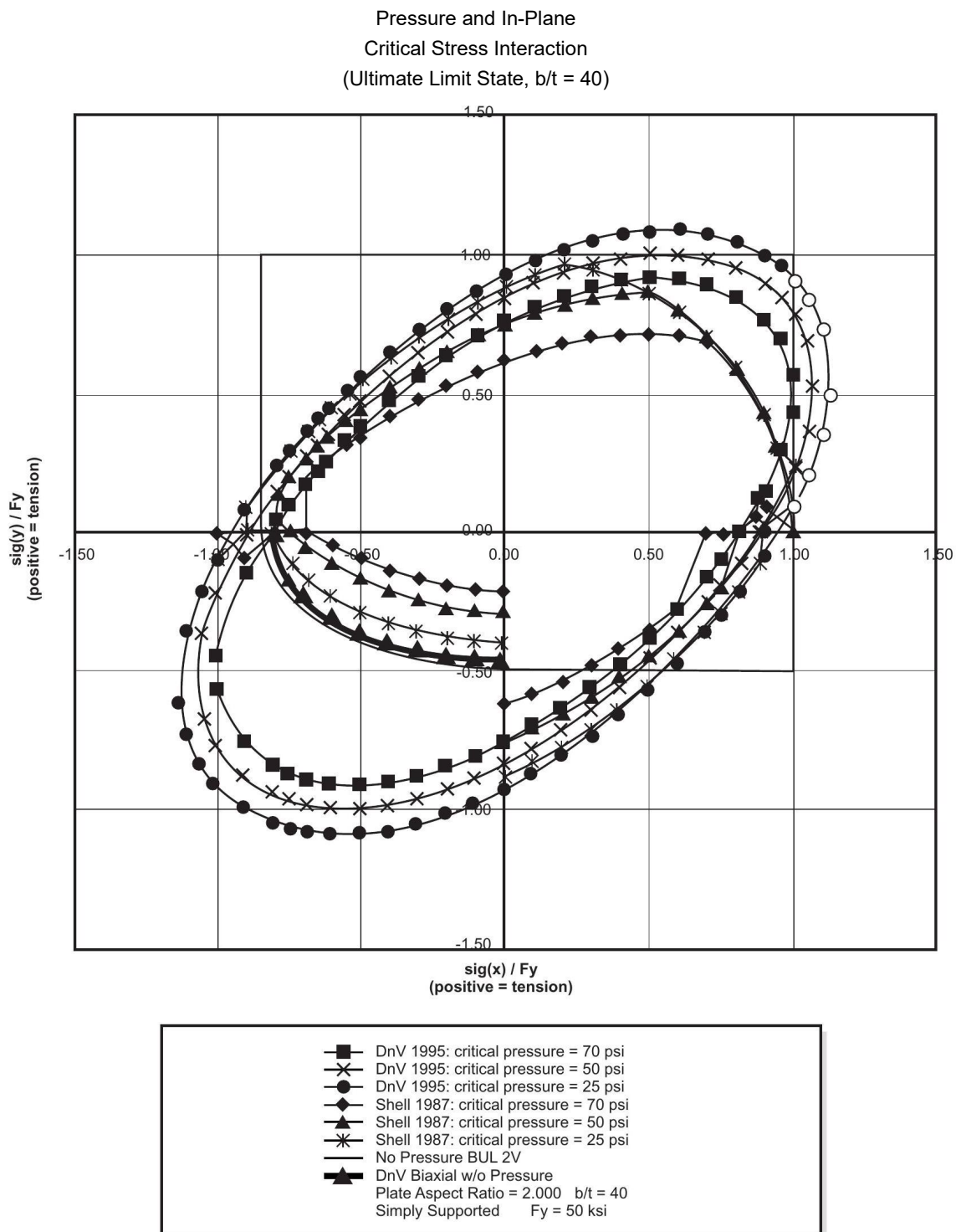
Figure C5-10—Combined In-Plane and Lateral Loads ( b/t = 40 )
