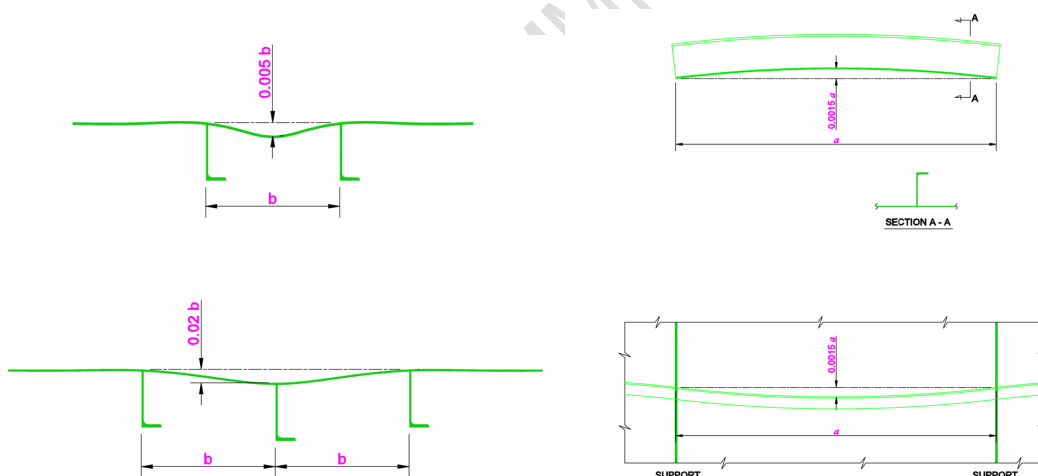
Figure 4.1-1—Construction Tolerance
