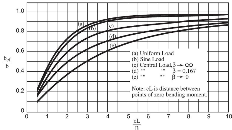
Figure 7.6-3—Effective Breadth Ratio for Case II (Double Web)*
