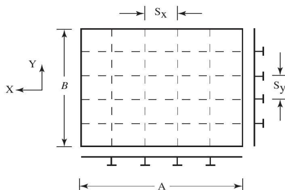
Figure 7.1-1—Flat Stiffened Panel
