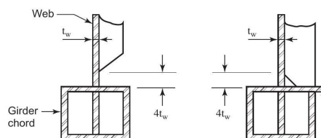
Figure 8.3-3—Vertical Stiffener Termination
