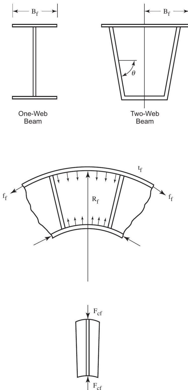
Figure 8.1-4—Transverse Stresses in Webs Due to Flanges Curved in Elevation
