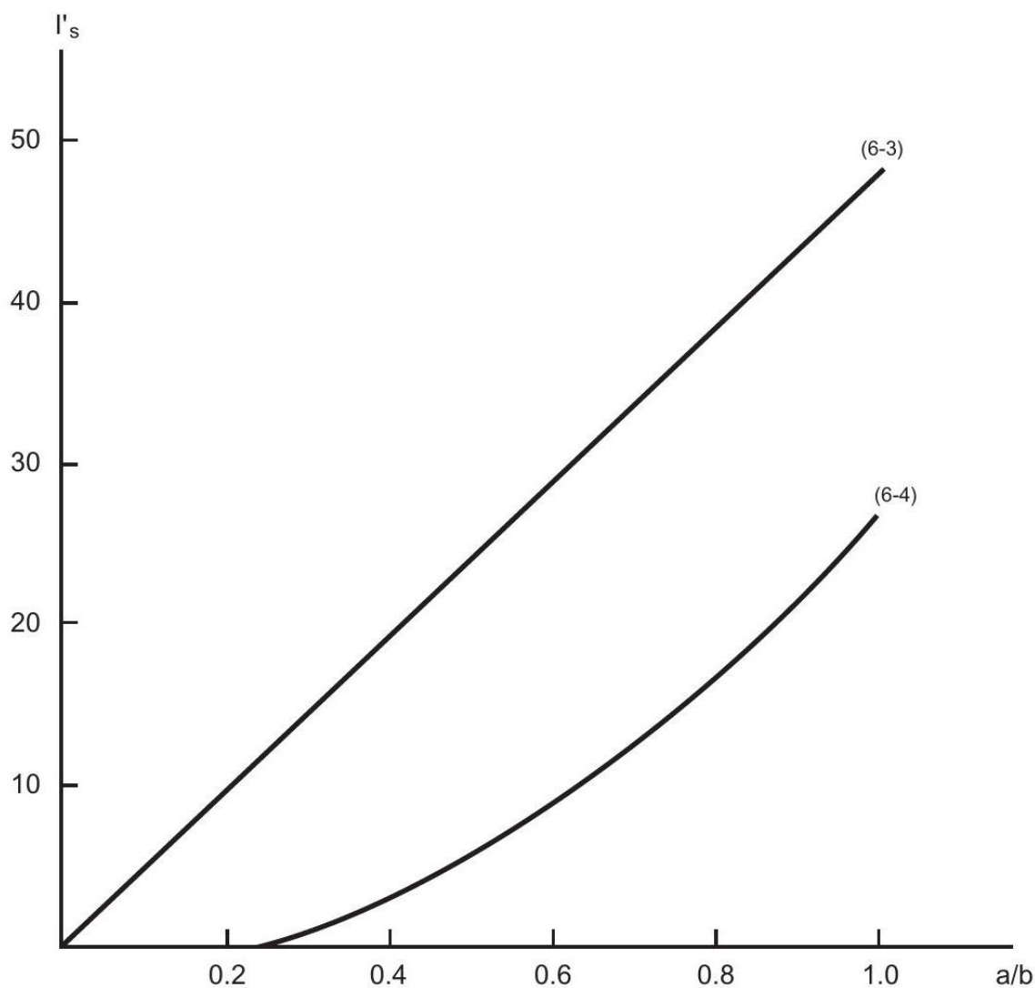
Figure C8-1-Comparison of Minimum Longitudinal Stiffener Stiffness Requirements
