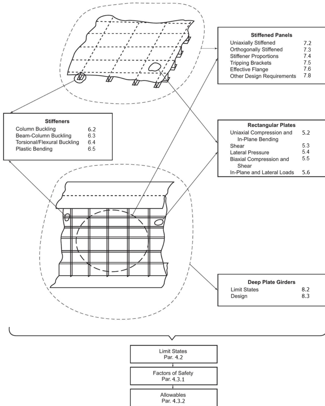
Figure 1-1 — Structural Components and Limit States Covered in this Bulletin
