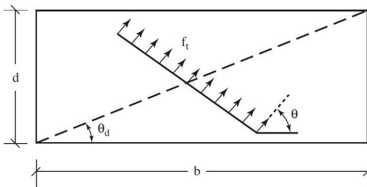
Figure C5-6—Model for the Ultimate Strength of Rectangular Plates in Shear
