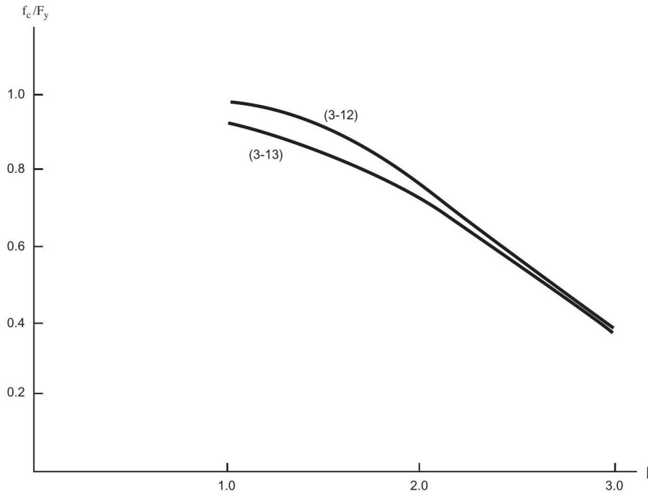
Figure C5-2-Comparison of Inelastic Buckling Formulations for Rectangular Plates Under Uniaxial Compression
