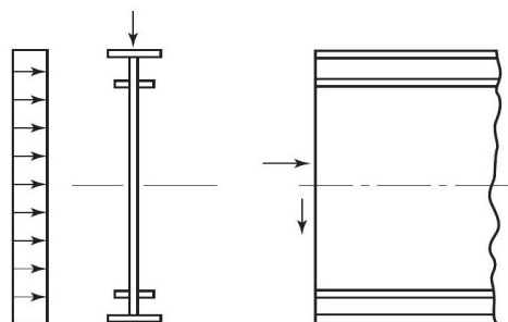
Figure 8.1-2—Primary Loads Acting on Plate Girder
