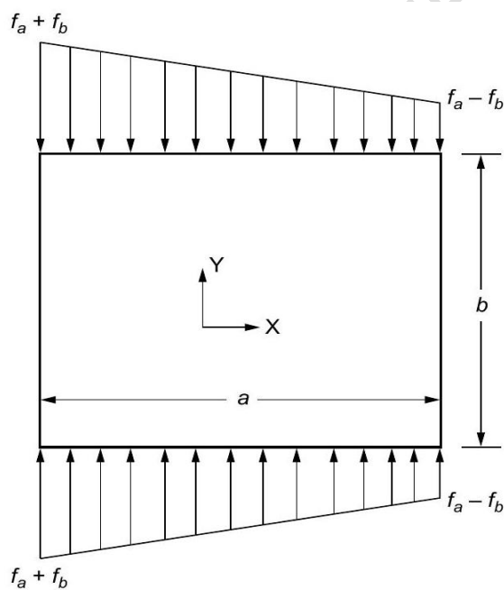
Figure 5.2-2—Wide Rectangular Plate
