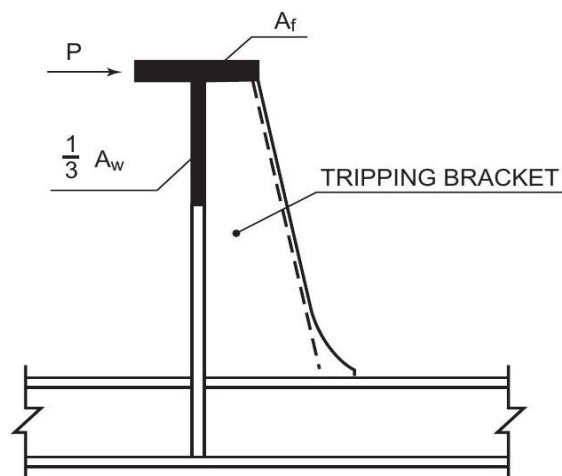
Figure 6.4-1—Design Lateral Load for Tripping Bracket
