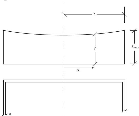
Figure 7.6-5—Stress Distribution Across Flange
