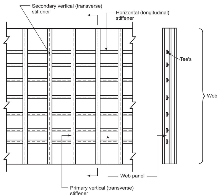
Figure 8.1-1—Typical Deep Plate Girder Structural Arrangement
