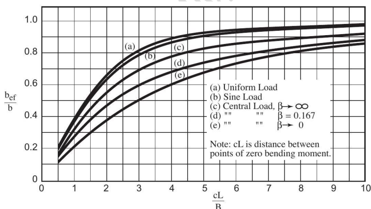
Figure 7.6-2—Effective Breadth Ratio for Case I (Single Web)*
