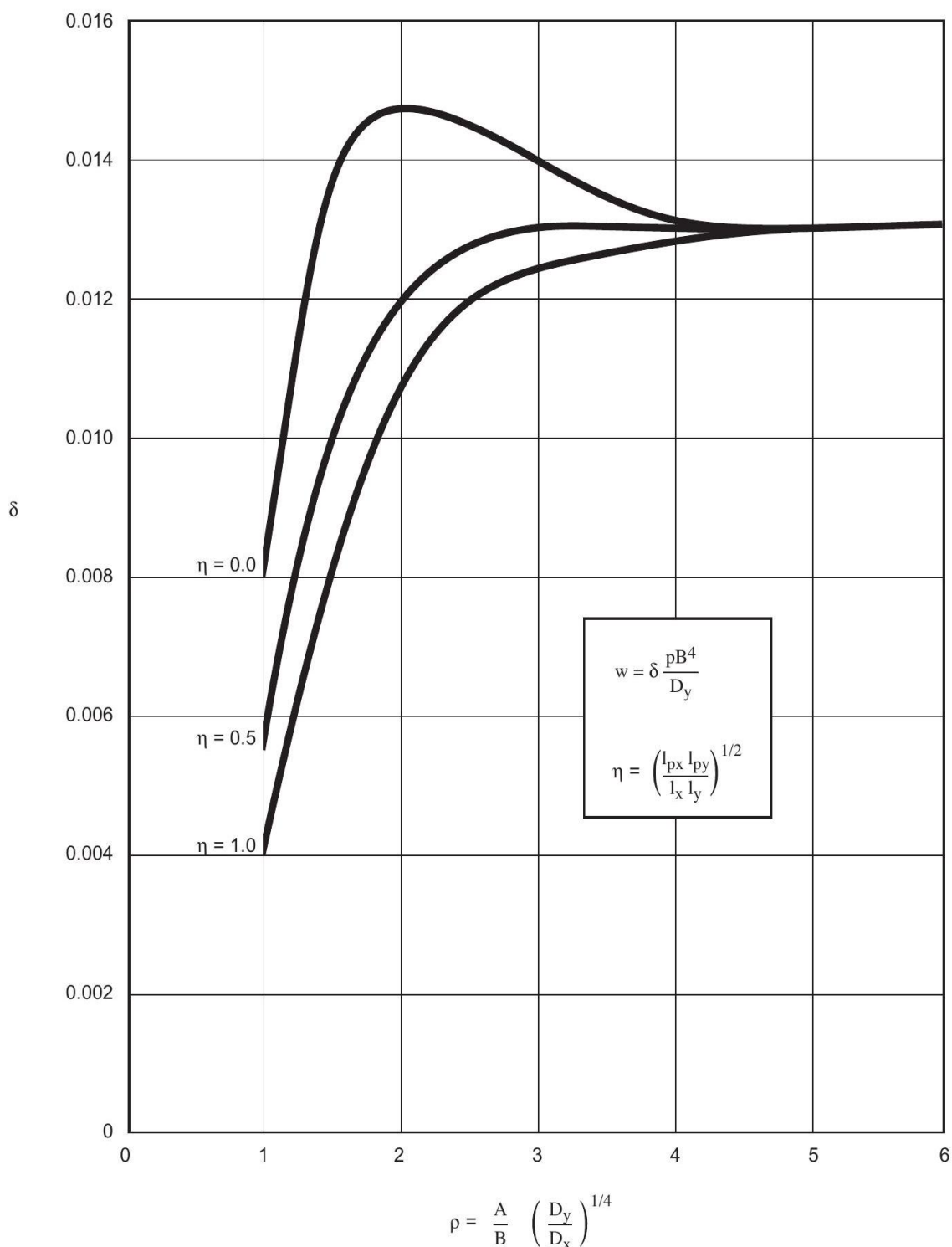
Figure 7.3-1—Deflection Coefficient for Orthogonally Stiffened Panels
