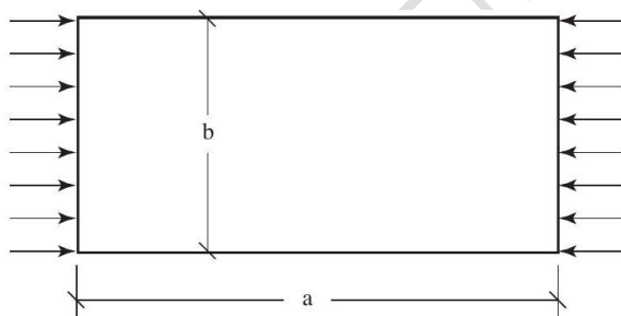
Figure C5-1—Rectangular Plate Under Uniaxial Compression
