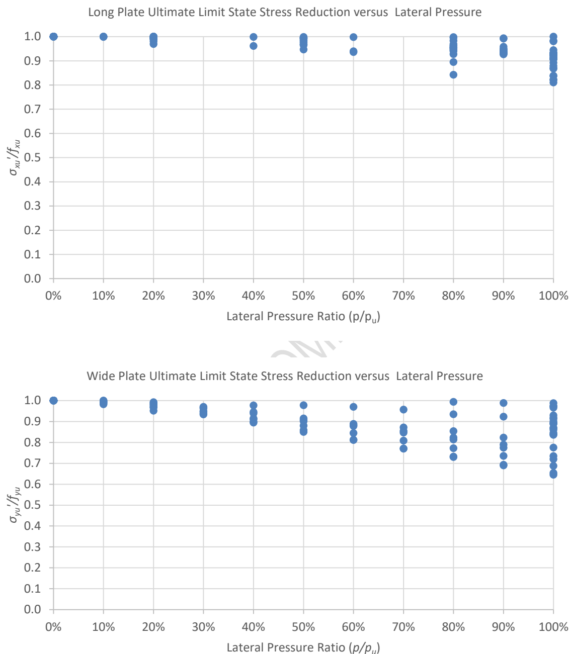
Figure C5-12—Long and Wide Plate In-Plane Stress versus Lateral Pressure
