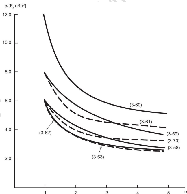
Figure C5-8—Comparison of Formulations for the Ultimate Strength of Rectangular Plates Under Lateral Pressure
