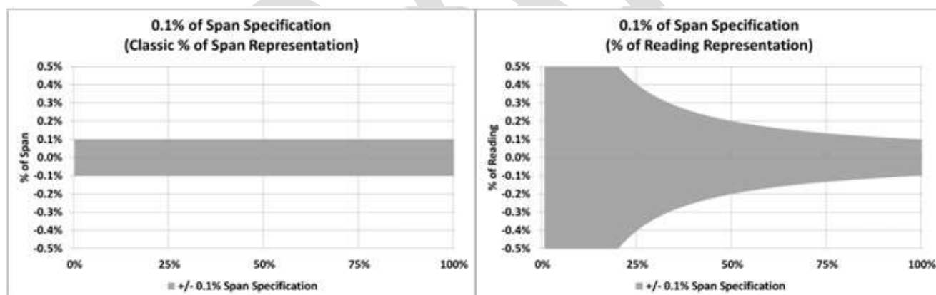
Figure A.1—Percentage of Span and Percentage of Reading Representation of a 0.1 % of Span Accuracy
