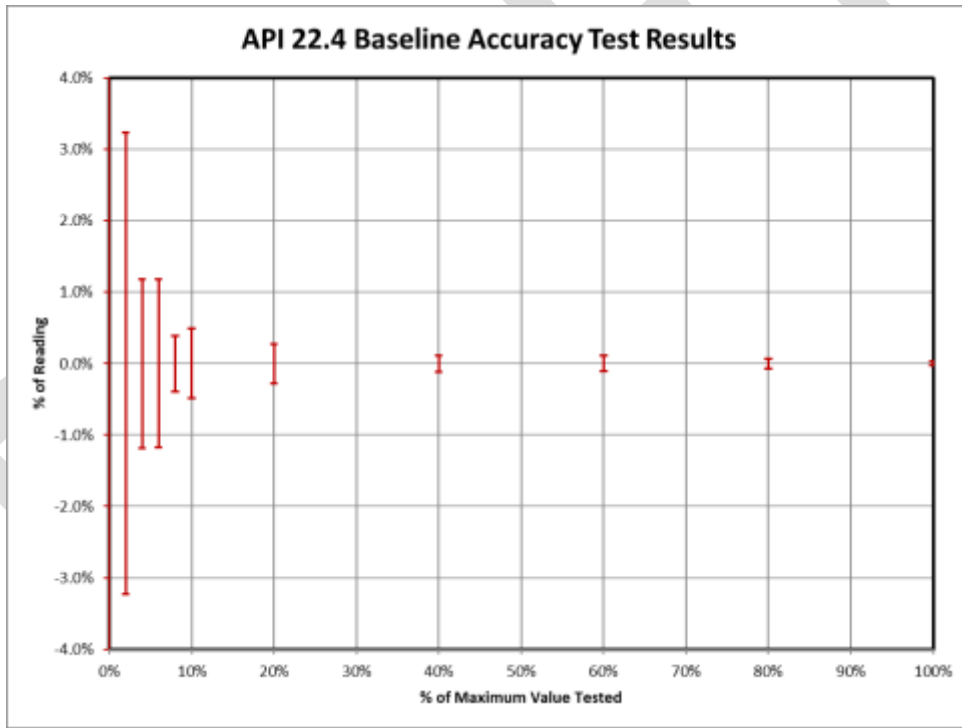
Figure 5—Section 6.4.1, API 22.4 Baseline Accuracy—Test Results
