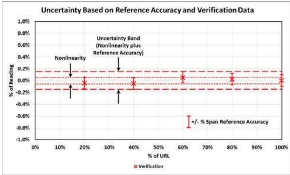
Figure A.6—Simplified API 22.4 Baseline Accuracy Nonlinearity and Uncertainty Based on Verification Data
