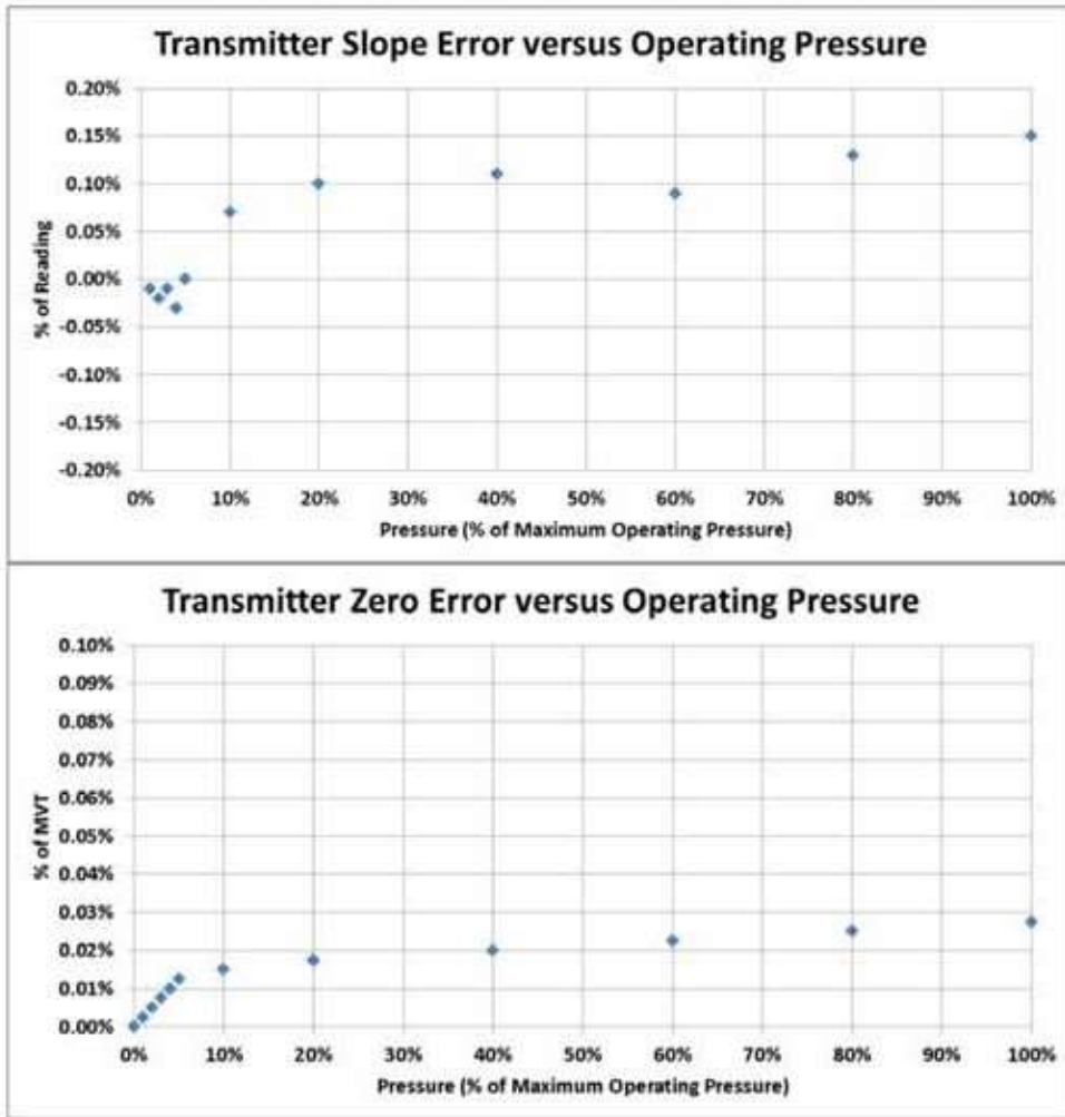
Figure 9—Section 6.5.3, Pressure Operating Effect on Differential Pressure Transmitter
